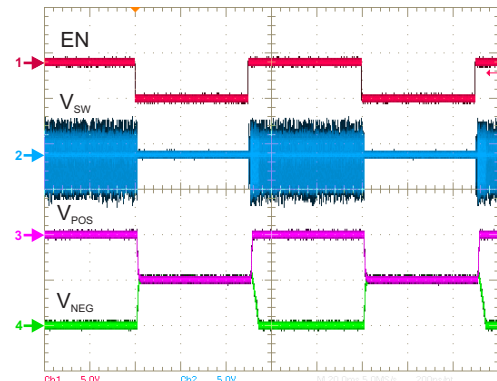
Figure 105. Power-Up/Down With Active Discharge — SYNC = HIGH
